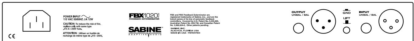
FBX-1020 Back Panel
